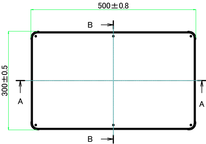
E view
